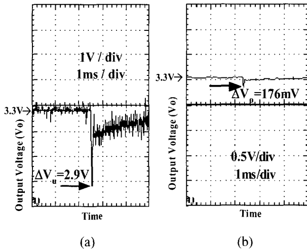
Fig. 13. Experiment results: Output voltage variation during steep load change,(a). Conventional topology ,(b).Proposed topology (Load change from 1A to 30A).
