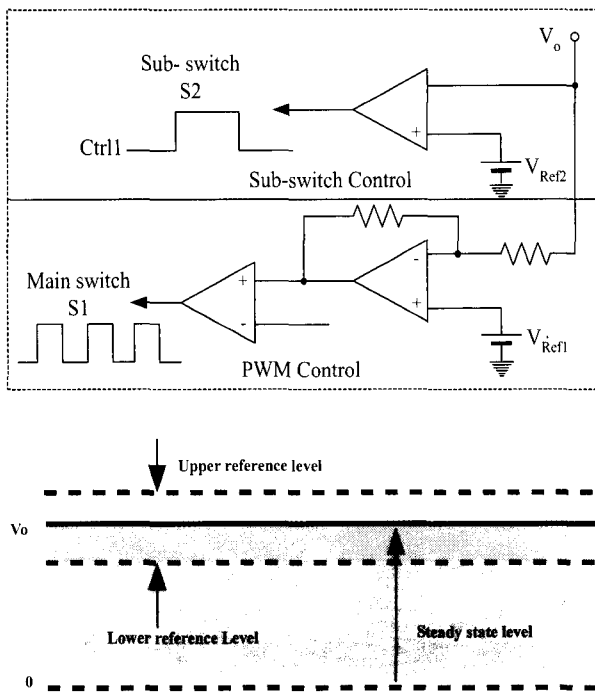
Fig. 11. Control scheme
