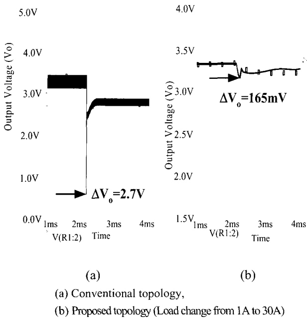
Fig. 12. Simulation results: Output voltage variation during steep load change.
