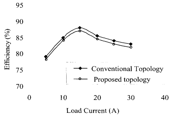
Fig. 14. Efficiency comparison.
