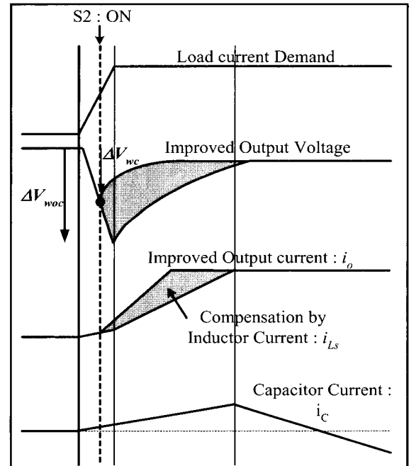
Fig. 10. Compensation of high-current clamp.
