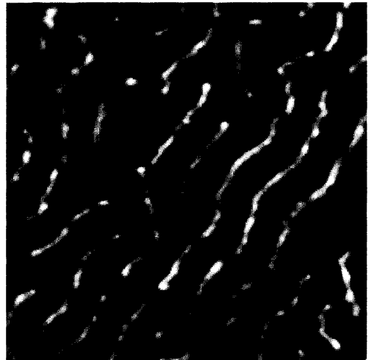
Fig. 8. MFM domain structure of (\text{Py-2 nm}/\text{Au-3 nm}/\text{Co-0.6 nm}/\text{Au-3 nm})_{15} multilayer in as-deposited state. The displayed area is 5 \mu\text{m} \times 5 \mu\text{m} .
