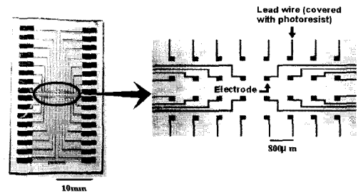
(a) 32 channels microelectrode array
