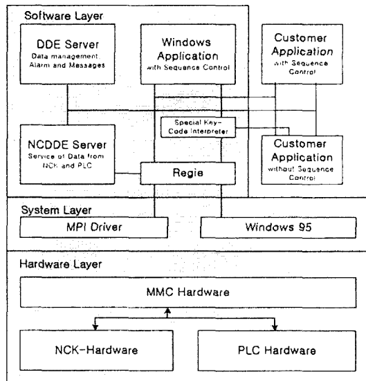
Fig. 3 MMC software organization
