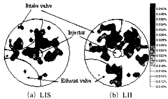
Fig. 6 Modified images of LIS and LII
