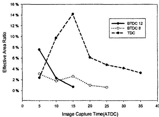
Fig. 11 Comparison of effective area ratio (LIS)
