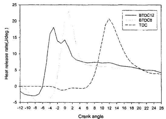
Fig. 9 Comparison of heat release rate (Injection: 12°, 8° BTDC, TDC, A/F=48, 400 rpm)
