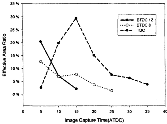
Fig. 10 Comparison of effective area ratio (LII)
