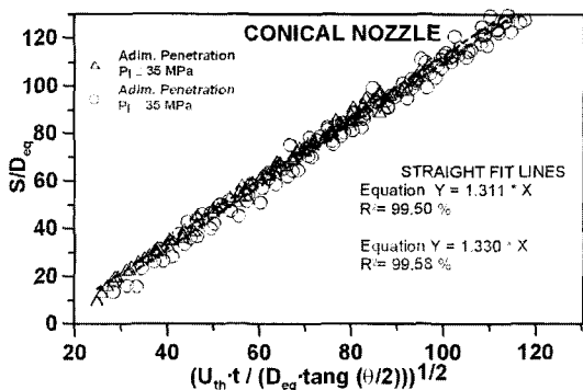
Fig. 10 Non-dimensional penetration for the conical nozzle
