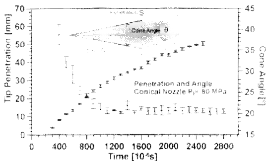
Fig. 5 Macroscopic parameters of the Spray. Mean values and the standard deviation for the conical nozzle, P_i=80 MPa
