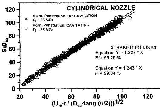
Fig. 9 Non-dimensional penetration for the cylindrical nozzle
