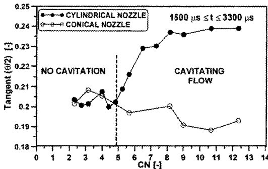
Fig. 8 Cone angle against the cavitation number
