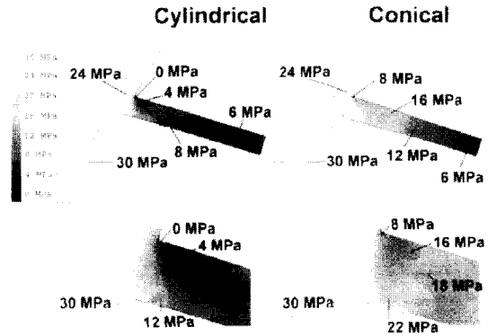
Fig. 4 Pressure field for the cylindrical and conical nozzle. P_i=30 MPa, P_b=6 MPa
