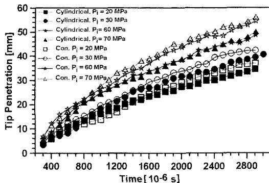
Fig. 6 Comparison of penetration between cylindrical and conical nozzle
