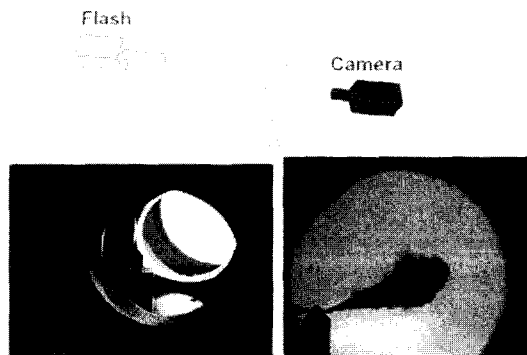
Fig. 2 Relative position of the flash, camera and injector. Sample of an image of a spray
