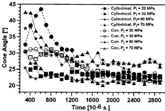
Fig. 7 Comparison of cone angle between cylindrical and conical nozzle
