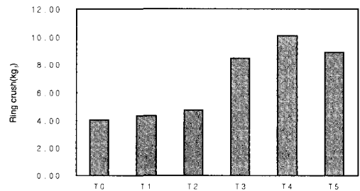
Fig. 7. Effect of application methods of water repellent agents and moisture proof agents on compressive strength of paper.
