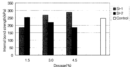
Fig. 3. Changes of internal bond strength of paper by starch insolubilizers(SI) dosage.
