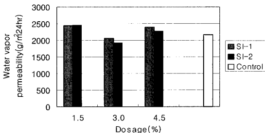
Fig. 2. Changes of water vapor permeability of paper by starch insolubilizers(SI) dosage.
