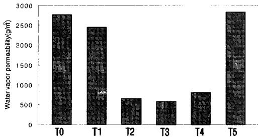
Fig. 8 Effect of application methods of water repellent agents and moisture proof agents on water vapor permeability of paper.
