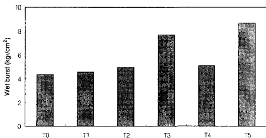
Fig. 6. Effect of application methods of water repellent agents and moisture proof agents on burst strength of paper.
