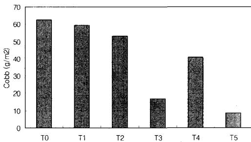
Fig. 5. Effect of application methods of water repellent agents and moisture proof agents on water absorbency of paper.
