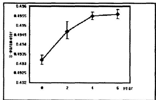
Fig. 4. S-parameters on the medical X-ray dose intensity in Gd_2O_3 : Tb screen vs. various years.
