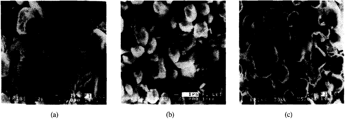
Fig. 3. SEM Photographs of large size grains in Gd_2O_3 : Tb (a) unexposed (b) exposed samples by 6 MV 6 Gy and (c) 15 MV 9 Gy X-ray
