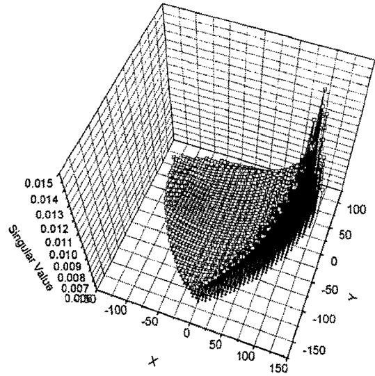
Fig. 6 \sigma_{min} in whole constant-orientation workspace
