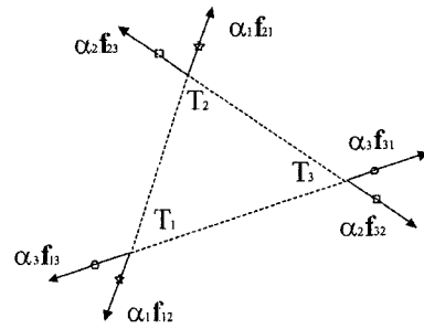
Fig. 4 Self-canceling internal forces at three EE points on mobile platform
