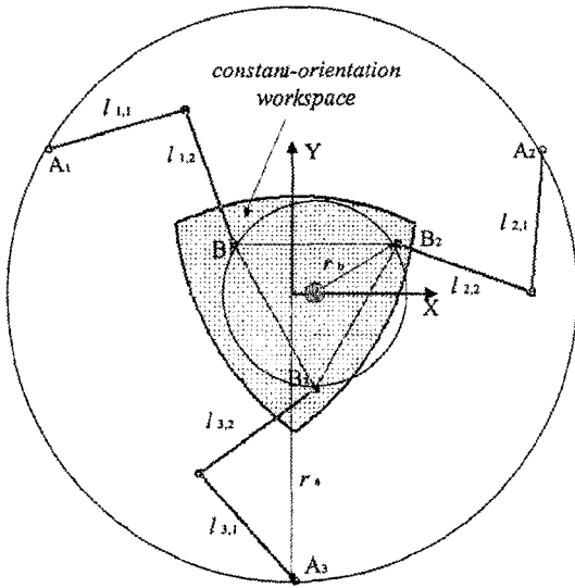
Fig. 5 Constant-orientation workspace for 3-RRR parallel manipulator
