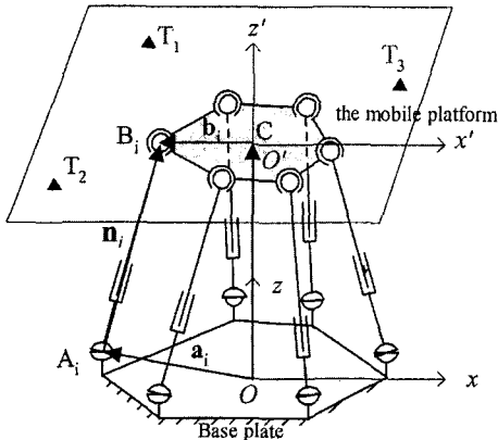
Fig. 1 6-6 General parallel manipulator (GPM)
