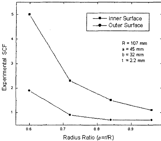
Fig. 3 Comparison of experimental SCF on inner and outer surface
