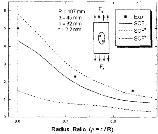
Fig. 5 SCF on the composite cylindrical shell with an elliptical cutout
