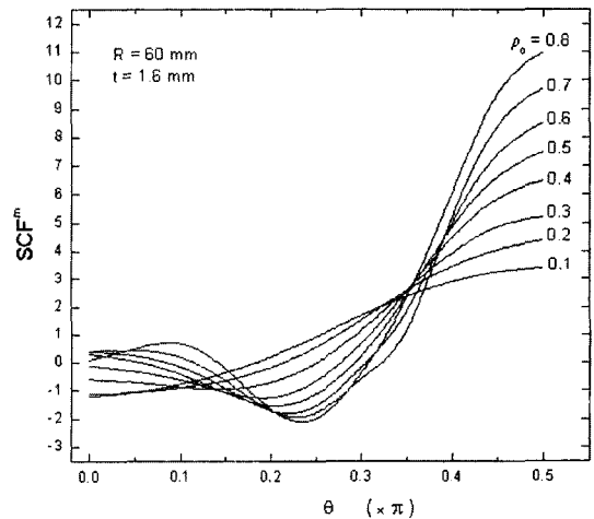
Fig. 6 Membrane SCF on various circular cutout size
