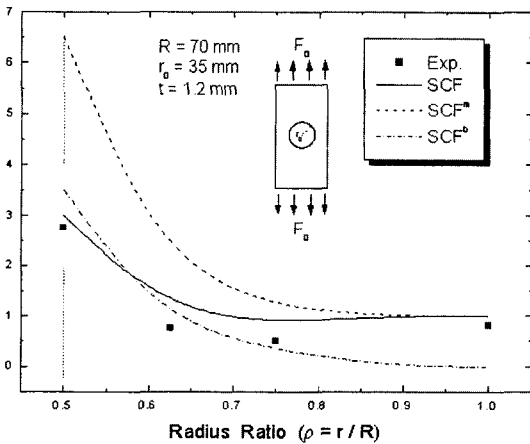
Fig. 4 SCF on the composite cylindrical shell with a circular cutout
