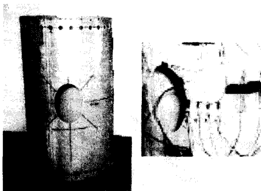
Fig. 2 Composite cylindrical shell having an elliptical cutout and strain gages attached around the cutout edge
