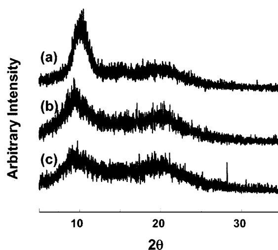
Figure 3. WAXD patterns of dermal scaffolds. (a) Chitosan, heat treated chitosan for (b) 1 day, and (c) 3 days.
