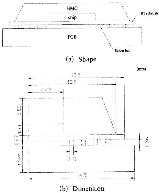
Fig. 1 Schematics of 256-pin PBGA-P package
