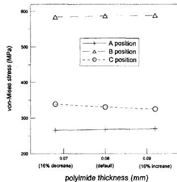
(c) von-Mises stress vs. polyimide thickness
