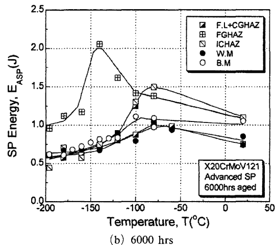
Fig. 9 SP energy transition behaviors for various micro-structures of virgin (a) and 6000 hrs aged material (b) in ASP test
