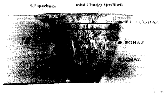
(a) Machining position and direction
