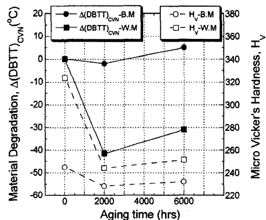
Fig. 8 Variation of \Delta(\text{DBTT})_{\text{CVN}} and micro Vicker's hardness
