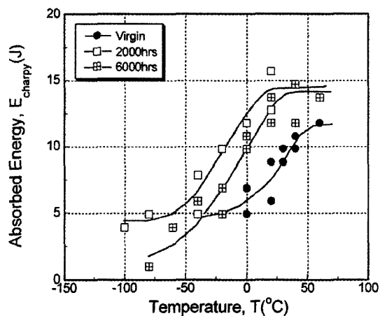
Fig. 7 CVN impact absorbed energy of WM
