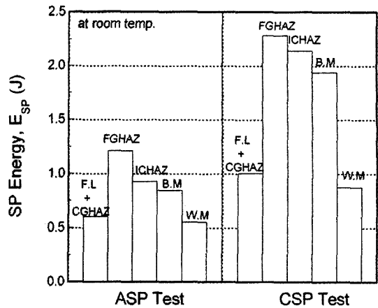
Fig. 5 A comparison of ESP from various micro-structures at R.T in SP test
