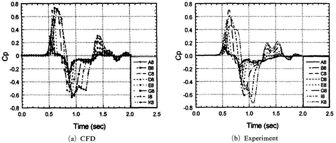
Fig. 5 Comparison of pressure coefficient curves from CFD with experiment
