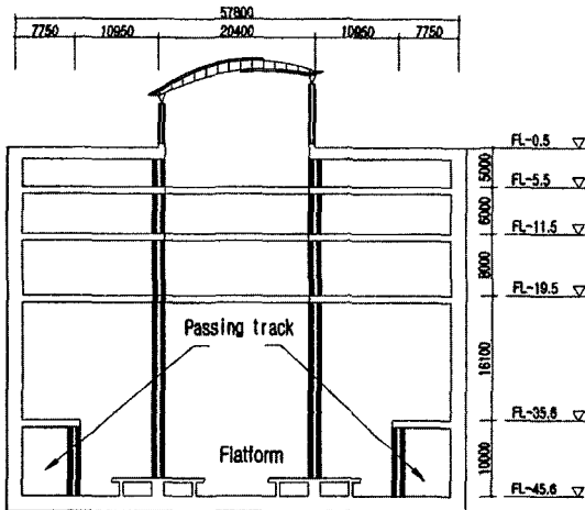
Fig. 3 A cross-section drawing of Daejeon station
