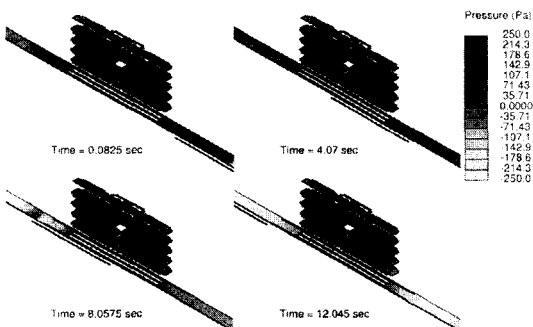
Fig. 9 Pressure distributions at the floors of Daejeon station
