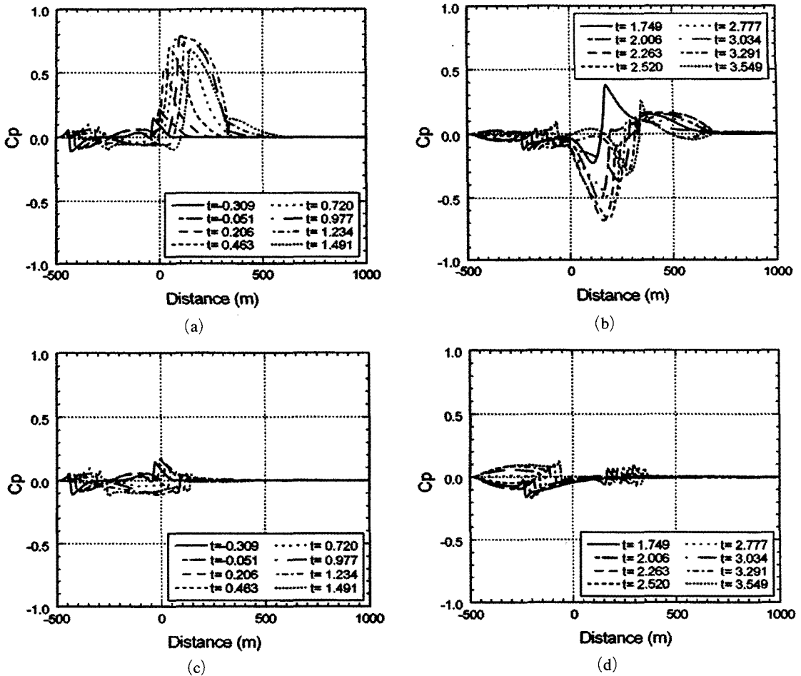
Fig. 10 Pressure transients at locations of tunnel ceiling height as HST passes through Daejeon station : (a), (b) With tunnel ; (c), (d) Without tunnel
