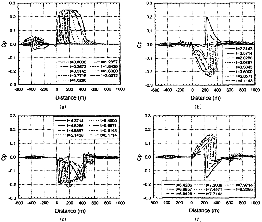
Fig. 8 Pressure transients at locations of tunnel ceiling height as HST passes through Gwangmyeong station
