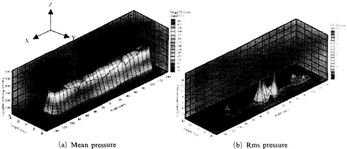
Fig. 5 Suction pressure distribution for the original suction nozzle
