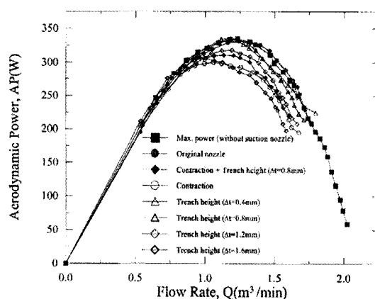
(a) Aerodynamic power
