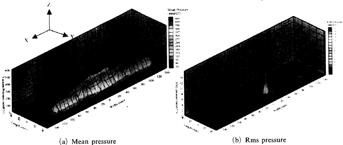
Fig. 7 Suction pressure distribution for connecting chamber modification
