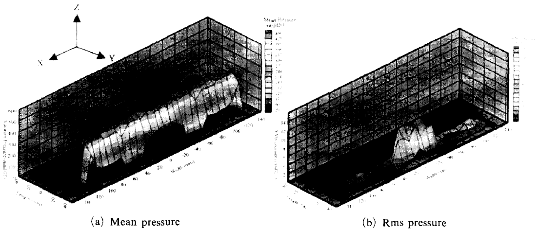
Fig. 6 Suction pressure distribution for the modified suction nozzle with trench height ( \Delta t=0.8 mm)
