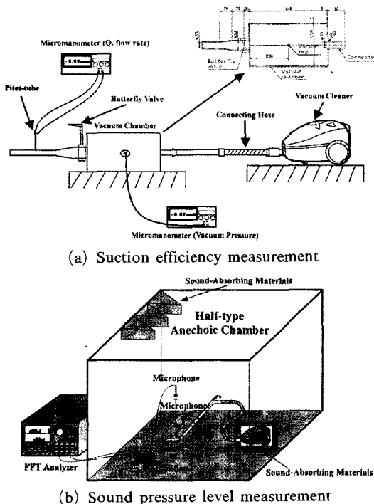
Fig. 1 Schematic diagram of experimental set-up for the suction efficiency and sound pressure level measurements
