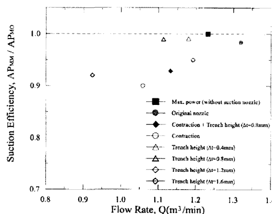
(b) Suction efficiency
