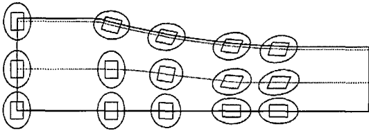
Fig. 13 Changes of grain shapes during cryogenic rolling at 196K
