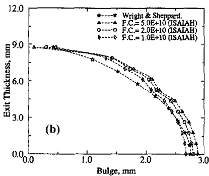
Fig. 9 Bulge profile at the exit plane for the bar rolling of (a) 10% and (b) 30% reduction
