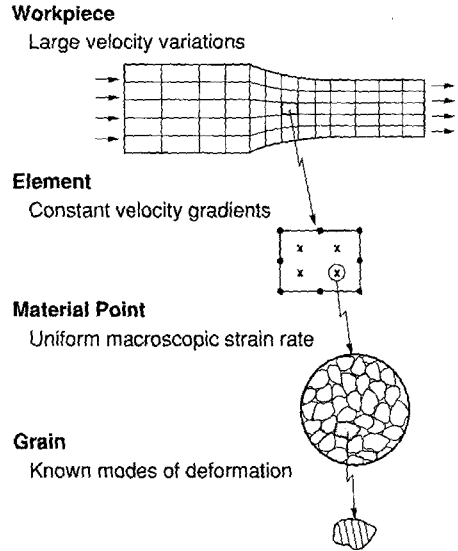
Fig. 1 Length scales in rolling simulation
