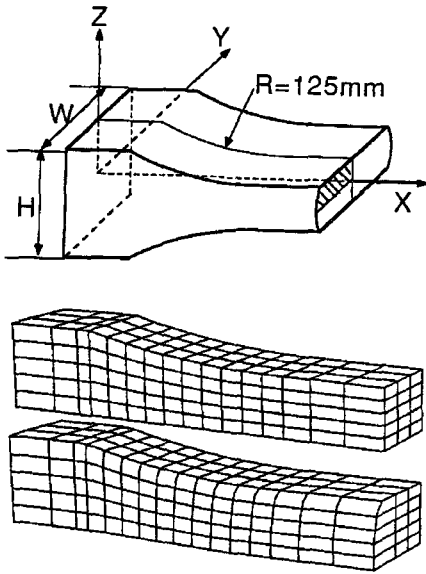
Fig. 8 Schematic of a bar rolling process and Eulerian finite element meshes before and after free surface correction
