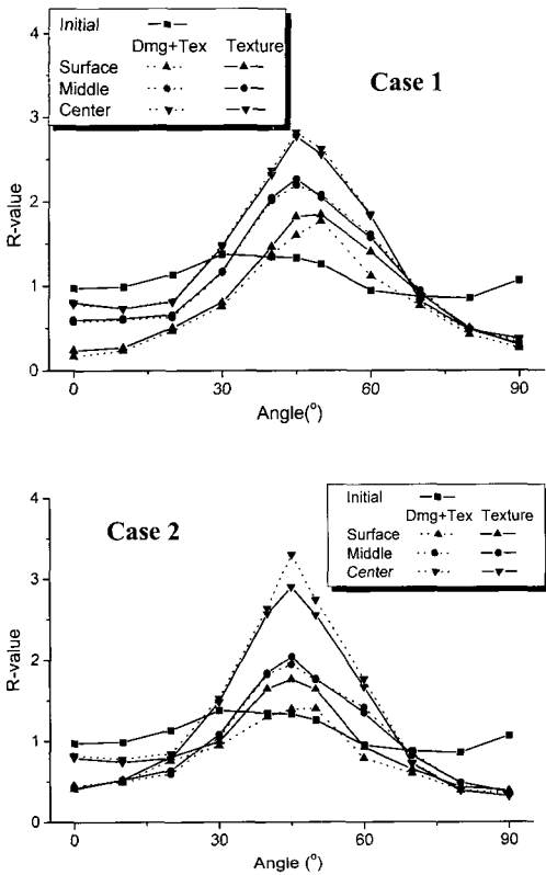
Fig. 6 Through-thickness R-values in Case 1 and Case 2
