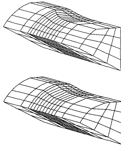
Fig.10 TRS rolling meshes before and after free surface correction
