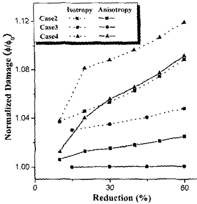
Fig. 2 Normalized damage along a centerline
