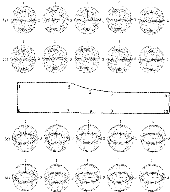
Fig. 5 Texture evolution in the final pass of case 2 : (a),(d)-Texture, (b),(c)-Damage+Texture
