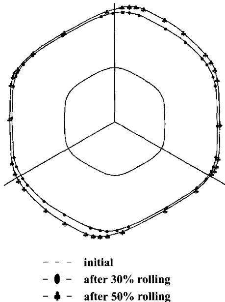
Fig. 7 Changes of yield surface during plate rolling with initial random texture
