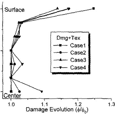
Fig. 3 Accumulated damage through thickness direction
