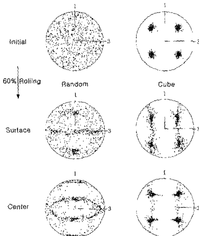
Fig. 4 {111} Pole figure for case 2
