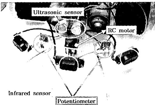
Fig. 3 Sensors for "RoJi"
