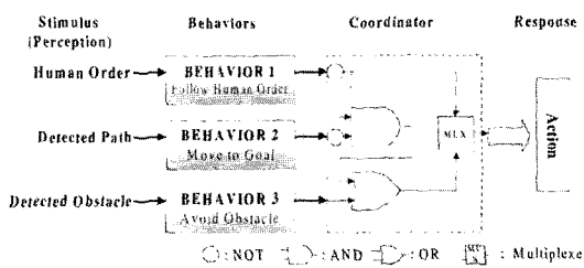
Fig. 8 A heuristic navigation strategy coordinator
