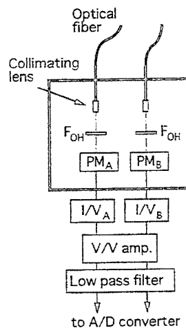
Fig. 3 Configuration of detection unit of the MICRO system
