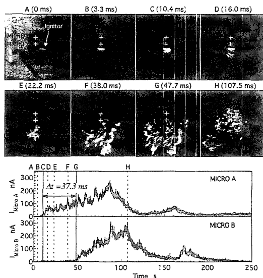
Fig. 7 Time-series data of OH chemiluminescence images recorded by the high speed CCD camera and local OH chemiluminescence monitored by the two MICRO systems
