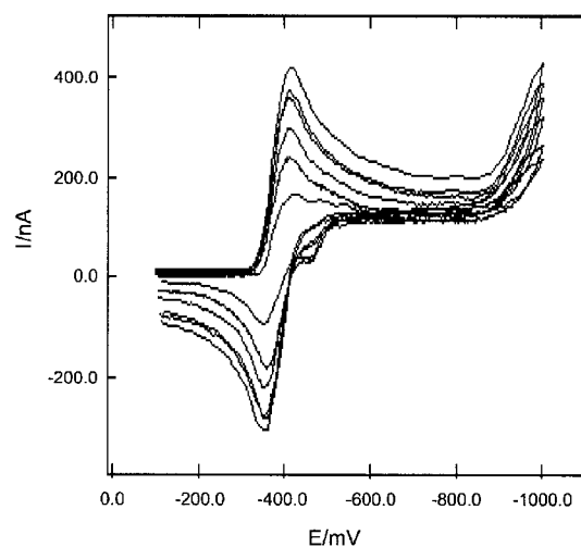
Fig. 2. The CVs of 1.0 \times 10^{-4} M doxorubicin hydrochloride in the acetate buffer of pH 3.5. Working electrode: HMDE, Electrode area: 0.0284 cm 2 , Equilibration: 20 sec, Initial potential: -0.1 V, Final potential: -1.0 V, Temperature: 23°C. Scan rates: 10 mV/s, 20 mV/s, 40 mV/s, 60 mV/s, 80 mV/s, and 100 mV/s (As the scan rates were increased, I_p^c and I_p^a were increased).
