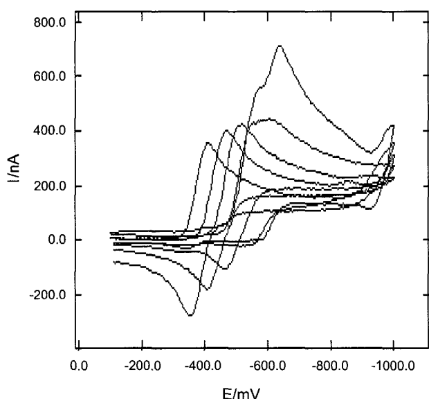
Fig. 3. The CVs of 1.0 \times 10^{-4} M doxorubicin hydrochloride in the acetate buffers of different pH values. From left to right: pH 3.5, pH 4.5, pH 5.5, pH 6.5, pH 7.5. Working electrode: HMDE, Electrode area: 0.0284 cm 2 , Equilibration: 20 sec, Initial potential: -0.1 V, Final potential: -1.0 V. Scan rate: 60 mV/s, Temp.: 23^\circ\text{C} .
