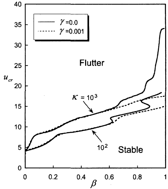
Fig. 5 Effect of internal damping on the critical flow velocity for k=100 and k=1000
