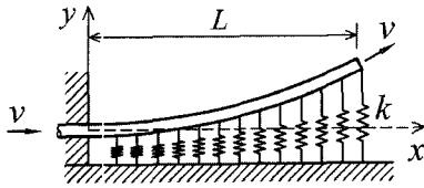
Fig. 1 Mathematical model of cantilevered pipe conveying fluid with elastic foundations
