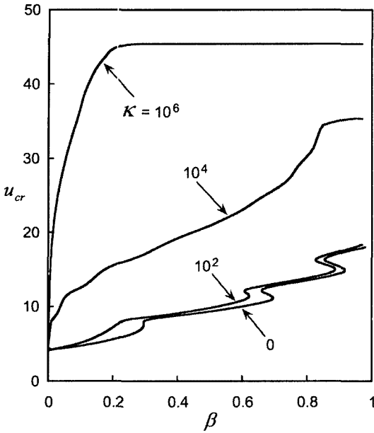
Fig. 3 Critical flow velocity depending on the mass ratio of the pipe and elastic foundation parameter ( r=0.0 )
