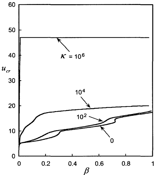
Fig. 4 Critical flow velocity depending on the mass ratio of the pipe and elastic foundation parameter ( r=0.001 )
