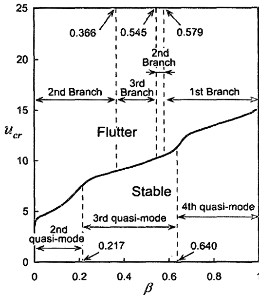
Fig. 10 Eigenvalue branches and quasi-modes depending on the mass ratio of the pipe \gamma=0.001 , K=100
