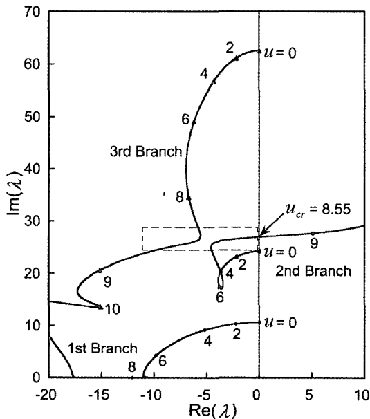
Fig. 7(a) Argand diagrams of the four lowest eigenvalues of the cantilevered pipes conveying fluid for \beta=0.300 ( \gamma=0.0, K=100 )
