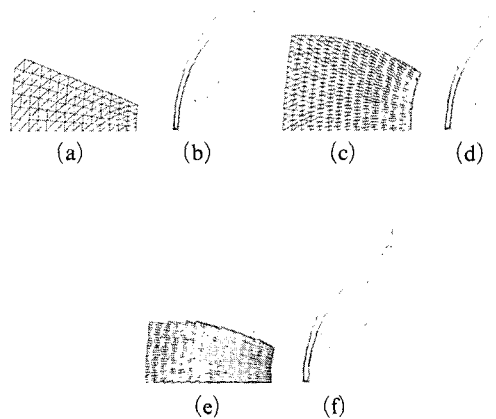
Fig. 6 Mach 15 flow over a blunt body, enlarged view of the mesh and computed density contours: (a)-(b) first mesh; (c)-(d) second mesh; and (e)-(f) third mesh
