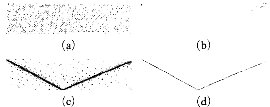
Fig. 12 An oblique shock reflection at a wall: (a)-(b) Initial mesh and the corresponding density contours; and (c)-(d) Third adaptive mesh and the corresponding density contours
