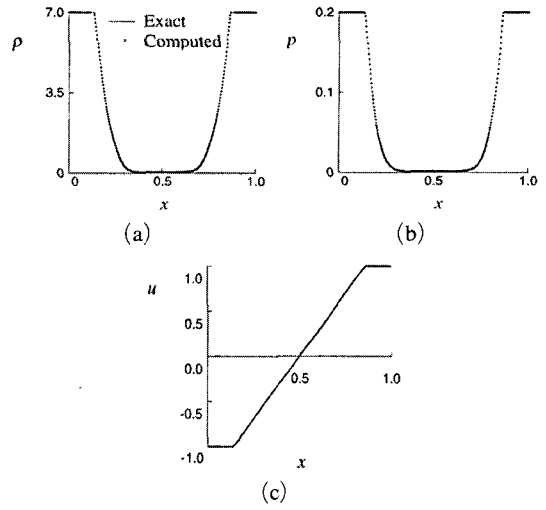
Fig. 10 Comparative exact and computed solutions at time t=0.3 for symmetric rarefaction wave problem \vartheta(2) : (a) density distributions; (b) pressure distributions; and (c) u -velocity distributions
