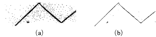
Fig. 15 Mach 2 flow in a 15^\circ channel \vartheta(1) : (a) Third adaptive mesh ; and (b) Density contours
