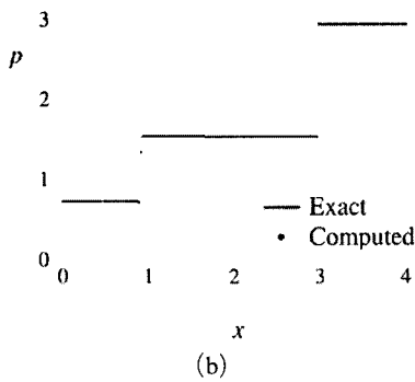
Fig. 13 Comparative solutions of an oblique shock reflection at a wall \vartheta(2) : (a) density distribution ; and (b) pressure distribution
