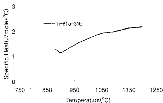
Fig. 6 Specific Heat of Ti-8Ta-3Nb alloys after T_\beta
