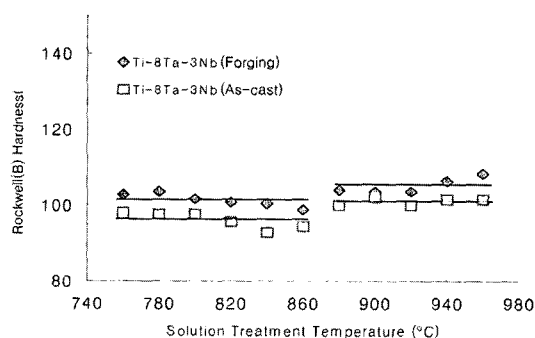
Fig. 1 Hardness test result after the solution heat treatment
