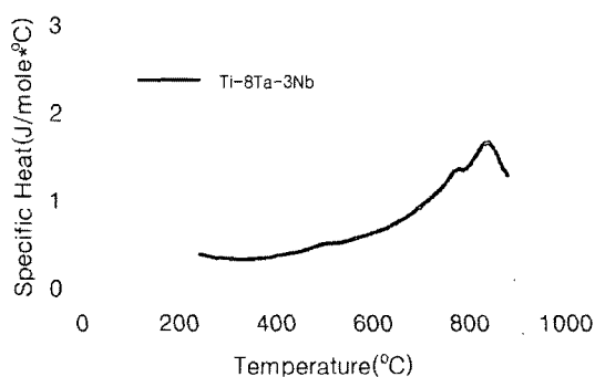
Fig. 5 Specific Heat of Ti-8Ta-3Nb alloys before T_\beta
