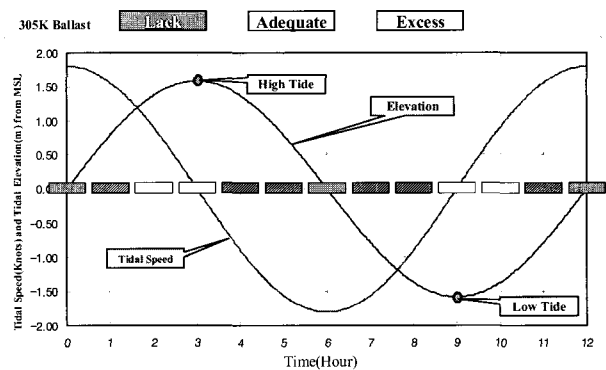
Fig. 9 Comparison of Estimated Optimum Tug Capacity and Guideline(305K VLCC-Ballast)
