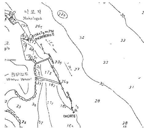
Fig. 1 VLCC Terminal in Gwang-Yang Harbor
