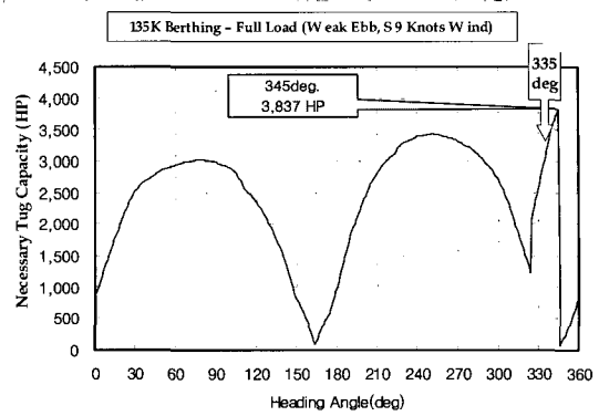
Fig. 5 Variation of Necessary Tug Capacity for Ship "O" with Heading Angle
