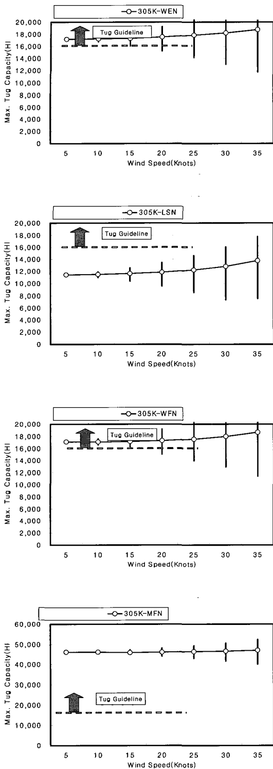
Fig. 7 Variation of Maximum Tug Capacity for 305K VLCC(Full Load - Berthing)
