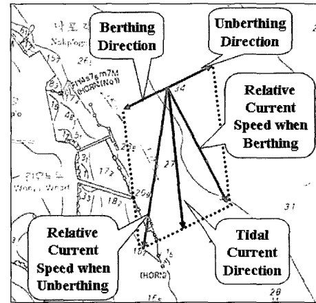
Fig. 3 Schematic Diagram of Relative Current Speed when Berthing or Unberthing
