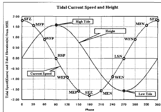
Fig. 6 Notation for Tidal Current Speed/Height Condition
