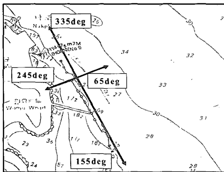
Fig. 2 Principal Direction of VLCC Terminal and Direction during Berthing/Unberthing
