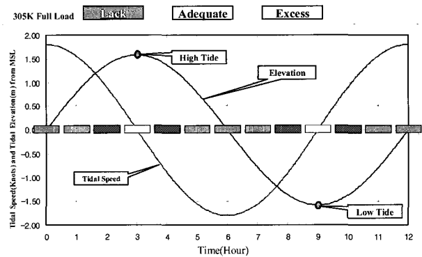
Fig. 8 Comparison of Estimated Optimum Tug Capacity and Guideline(305K VLCC-Full Load)
