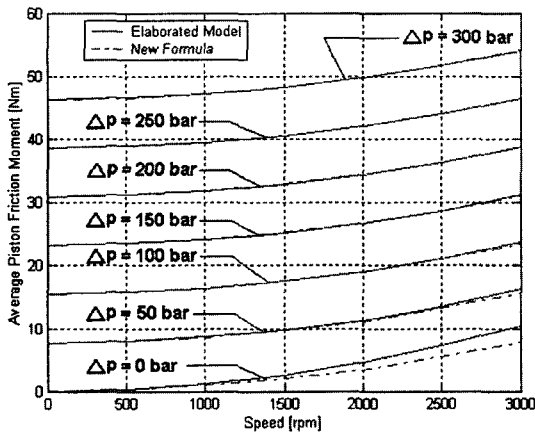
Fig. 9 New formula for average friction moment
