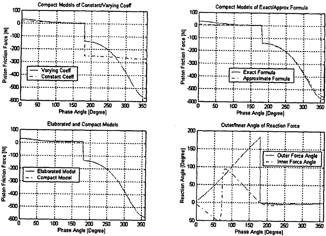
Fig. 6 Comparison of compact and elaborated models (no bushing)
