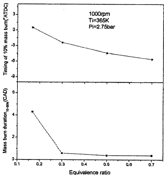
Fig. 6 Effect of equivalence ratio on combustion (propane)
