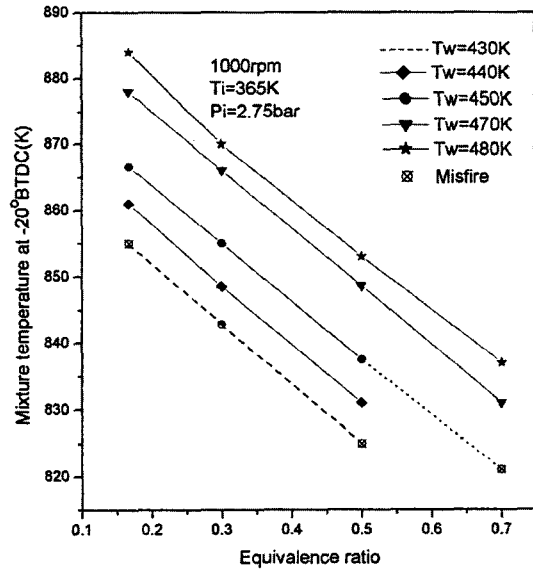
Fig. 8 Effect of equivalence ratio and wall temperature on compressed mixture temperature (propane)
