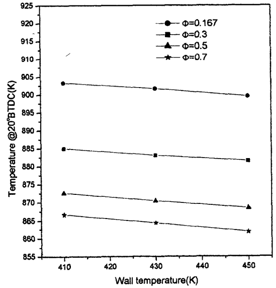
Fig. 10 Minimum compression temperature to autoignite at 20° BTDC for wall temperatures (propane ; 1000rpm and P_i=1\text{bar} )
