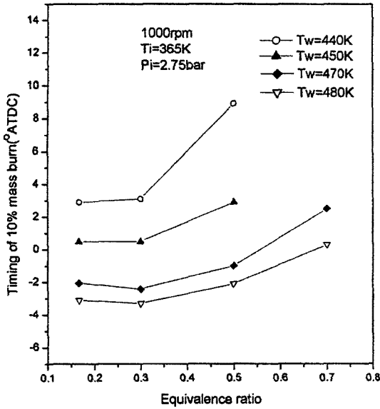
Fig. 7 Effect of equivalence ratio on combustion (propane) for fixed wall temperatures
