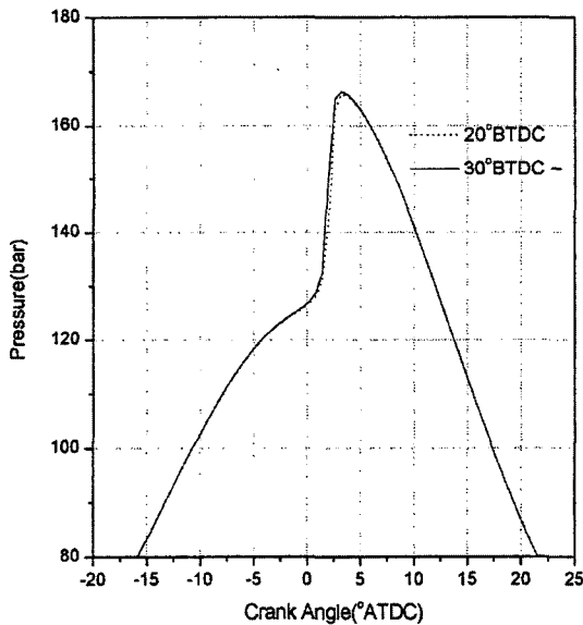
Fig. 2 Computed in-cylinder pressure traces for different timings to activate chemical kinetics
