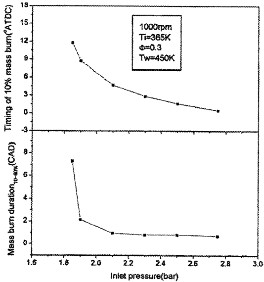
Fig. 5 Effect of intake pressure on combustion duration (propane)
