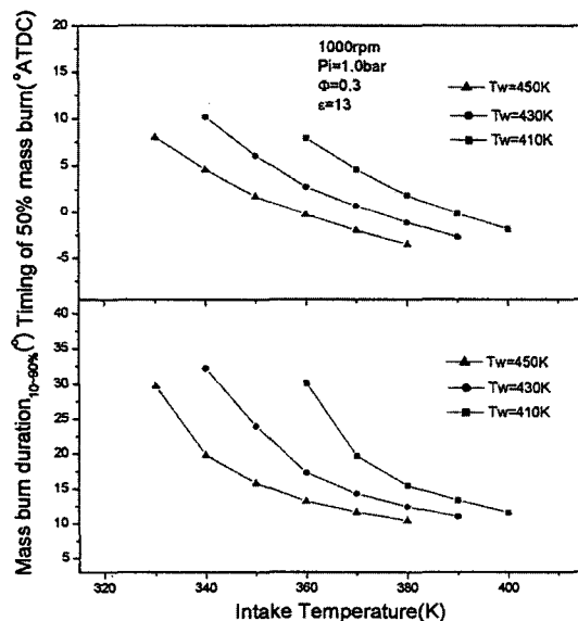
Fig. 12 Effect of intake temperature and wall temperature on combustion (n-heptane)
