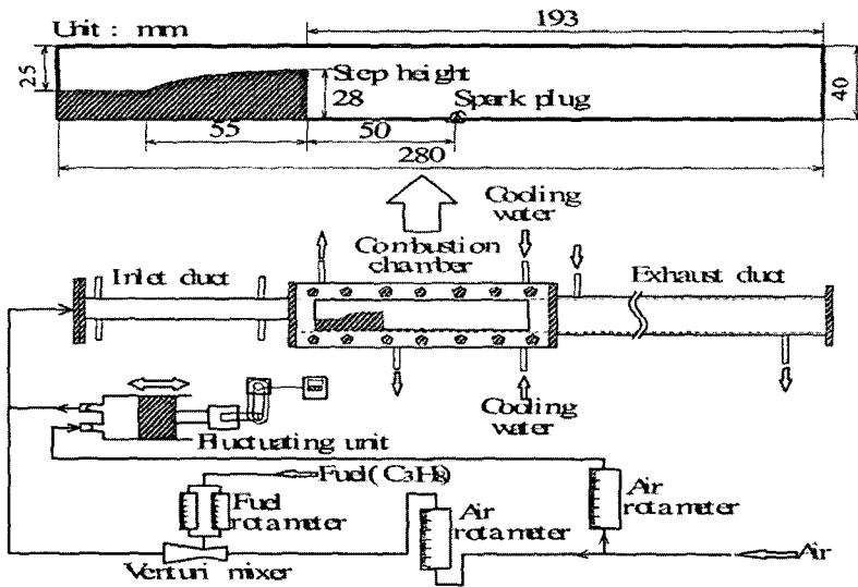
Fig. 1 Experimental apparatus
