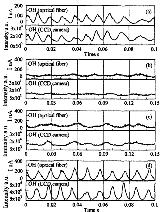
Fig. 3 Signals obtained by optical fiber and CCD camera, (a) Combustion oscillation with constant mixture supply, L_d=600\text{mm} , \phi=0.8 , (b) No oscillation with constant mixture supply, L_d=900\text{mm} , \phi=0.7 , (c) No oscillation suppressed with forced oscillating mixture supply, L_d=900\text{mm} , \phi=0.75 , (d) Intense combustion oscillation with constant mixture supply, L_d=900\text{mm} , \phi=1.0 .
