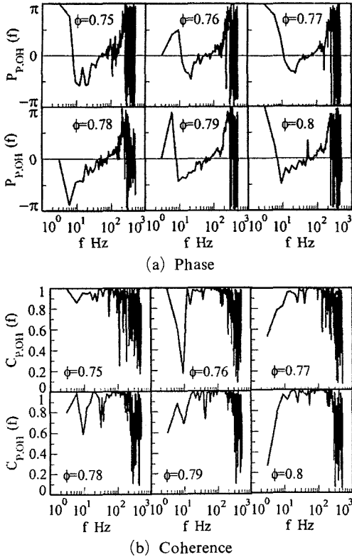
Fig. 8 Phase and coherence between pressure and OH in FFT with fine base frequency
