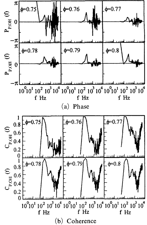
Fig. 9 Phase and coherence between pressure and OH in FFT with coarse base frequency
