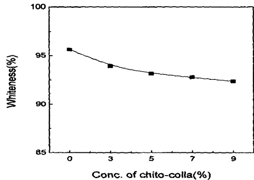
Fig. 2. whiteness of cotton fabrics by varying conc. of chito-colla.
