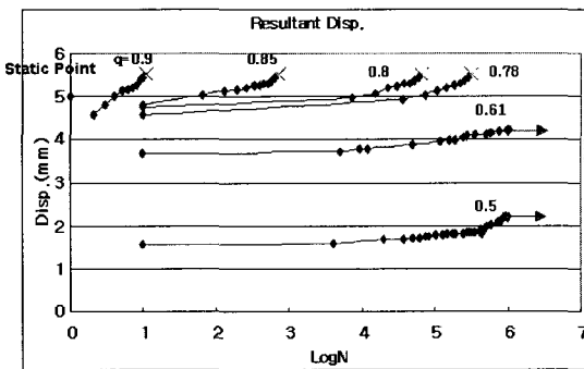
Fig. 12 Resultant displacement. versus cycles.
