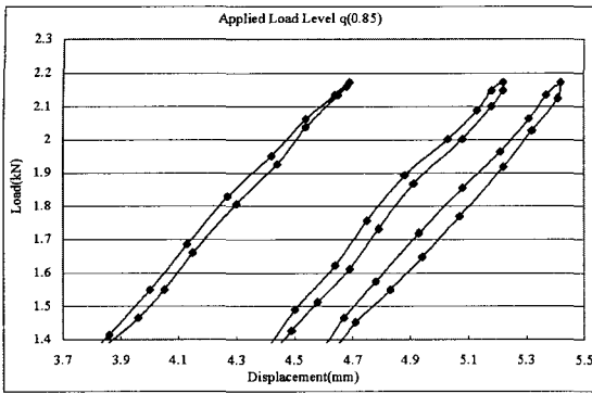
Fig. 10 Cyclic load-displacement of SAS.
