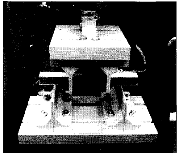
Fig. 8 Configurations of specimens & jig.
