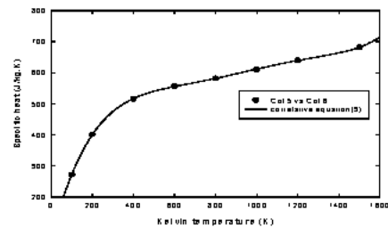
Fig. 3 Specific heat distribution with temperature variations for the STS 304 hollow cylinder
