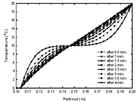
Fig. 9 Temperature distributions by time variation with constant properties at cross section for the STS 304 hollow cylinder
