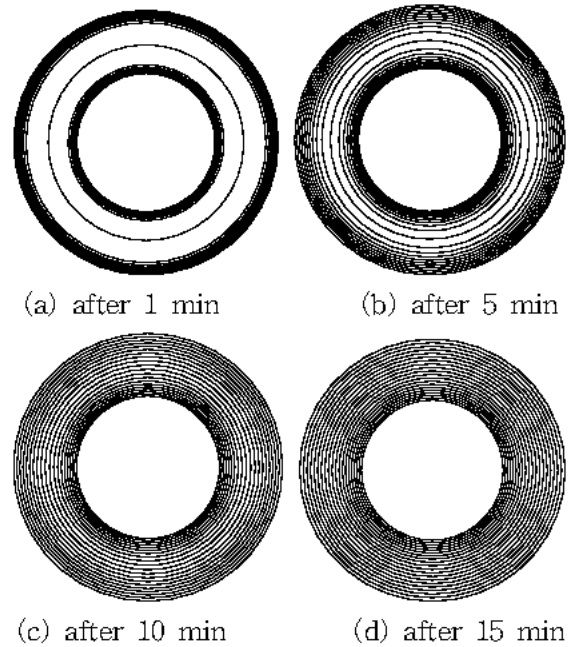
Fig. 8 Temperature contours by time variation with temperature-dependent specific heat and conductivity for the STS 304 hollow cylinder
