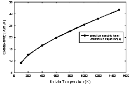
Fig. 4 Conductivity distribution with temperature variations for the STS 304 hollow cylinder
