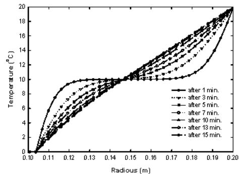
Fig. 11 Temperature distributions by time variation with temperature-dependent conductivity at cross section for the STS 304 hollow cylinder
