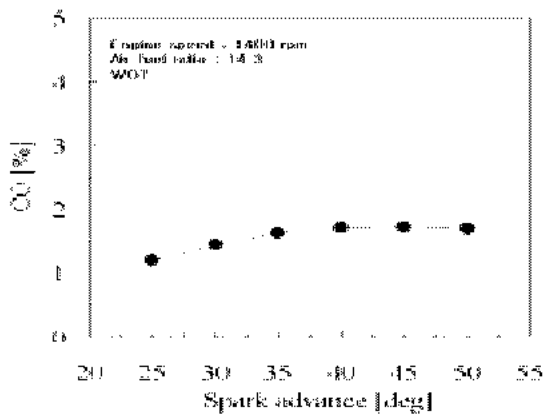
Fig. 3 Variation of the carbon monoxide concentration with respect to the spark advance of spark ignition engine
