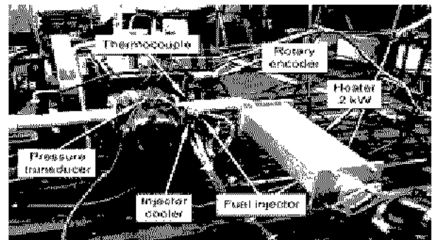
Fig. 2 Photograph of engine
