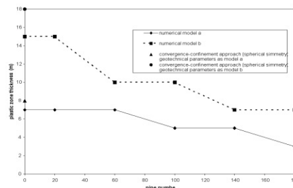
Fig. 3 Plastic zone ahead the tunnel face along the tunnel axis for the carried out analyses
