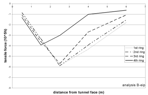
Fig. 6a Stress distribution inside the pipes for the ideally elasto-plastic A and B analyses
