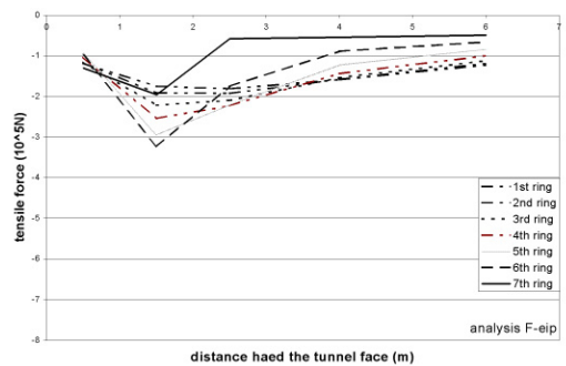
Fig. 6b Stress distribution inside the pipes for the ideally elasto-plastic E and F analyses
