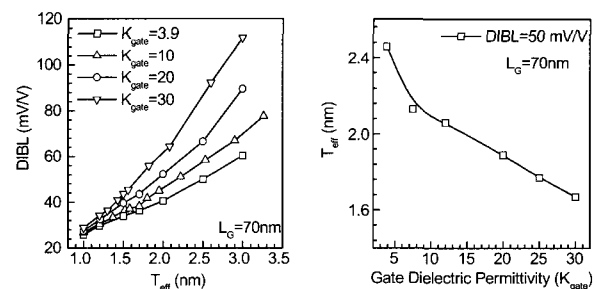
Fig. 13. DIBL as a function of effective gate dielectric thickness for different K_{\text{gate}} .
