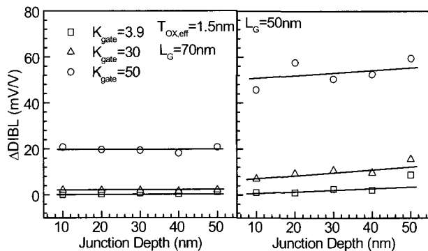
Fig. 9. The difference in DIBL between transistors having L_{\text{ov}} of 1nm and 12nm as a function of junction depth for different gate dielectric permittivity. The effective channel length and effective dielectric thickness of the transistors is kept fixed during simulation.
