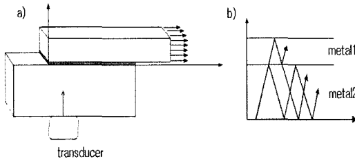
Fig. 5 Signal analysis classification of single lap joints
