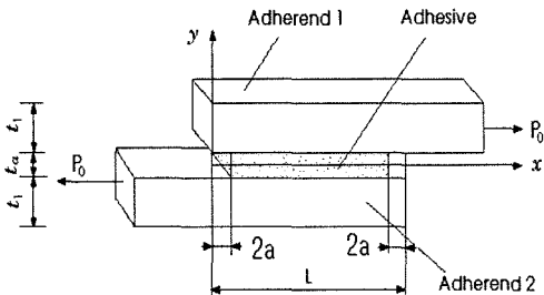
Fig. 1 Test specimen description of adhesively bonded lap joints
