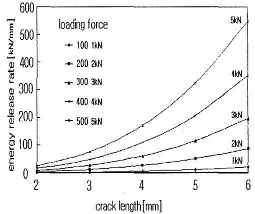
Fig. 4 Comparison of energy release rate vs. crack length
