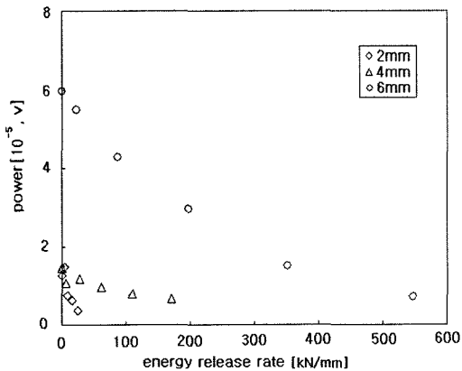
Fig. 9 Comparison of energy release rate vs. power
