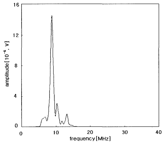
Fig. 7 Frequency vs. amplitude waveform by FFT
