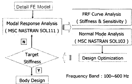
Fig. 10 The procedures of body attachment stiffness analysis
