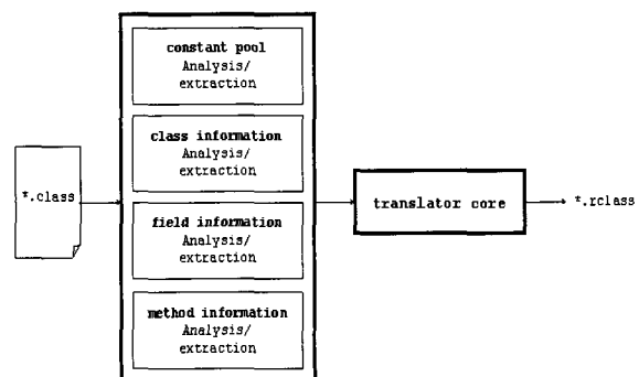
(Fig. 3) Java Class File Translator(from *.class to *.rclass)
