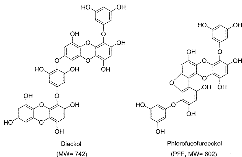
Fig. 1. Chemical structures of dieckol and phlorofucofuroeckol (PFF). By means of 1 H-NMR spectra and comparisons with published data, both dieckol and PFF were identified as shown in "Materials and Methods".
