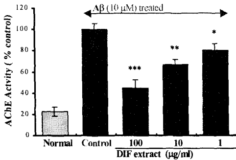
Fig. 8. Inhibitory effects of DIF extract on the AChE activity in Aβ stimulated PC-12 cells. Normal : Non-treatment group. Control : Group pretreated with 10µM Aβ for 1 hour. DIF I : Group pretreated with 10µM Aβ for 1 hour and 100µg/ml of DIF extract for 24 hours. DIF II : Group pretreated with 10µM Aβ for 1 hour and 10µg/ml of DIF extract for 24 hours. DIF III : Group pretreated with 10µM Aβ for 1 hour and 1µg/ml of DIF extract for 24 hours. * : Statistically significant value compared with control data by T test(* : p<0.05, ** : p<0.01, *** : p<0.001). PC-12 cell was pretreated with various concentration DIF extract(100, 10, 1µg/ml) in the presence Aβ(10µM) for 24hrs. The lysate(50µl) were measured using AChE diagnosis kits. The other methods for assay were performed as described in Materials and Methods .
