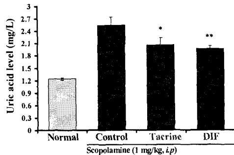
Fig. 10. Effects of DIF extract on the uric acid in the serum level of memory deficit rats induced by scopolamine. Normal : Non-treatment group. Control : Group treated with scopolamine(1mg/kg i.p). Tacrine : Group treated with scopolamine(1mg/kg i.p) and tacrine(10mg/kg p.o). DIF : Group treated with scopolamine(1mg/kg i.p) and DIF extract(150mg/kg p.o). * : Statistically significant value compared with control data by T test(* : p<0.05, ** : p<0.01, *** : p<0.001). SD rats were orally administered with DIF or tacrine and the injection of scopolamine(1mg/kg i.p) continued once a day for 7 days. Hematologic change was analyzed as described in Materials and Methods .
