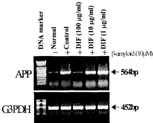
Fig. 2. Inhibitory effects of DIF extract on APP mRNA expression in PC-12 cell cultures after treatment with A \beta . Normal : Non-treatment group. Control : Group pretreated with 10 \mu M A \beta for 1hr. DIF I : Group pretreated with 10 \mu M A \beta for 1 hour and 100 \mu g/ml of DIF extract for 6hrs. DIF II : Group pretreated with 10 \mu M A \beta for 1 hour and 10 \mu g/ml of DIF extract for 6hrs. DIF III : Group pretreated with 10 \mu M A \beta for 1 hour and 1 \mu g/ml of DIF extract for 6hrs. PC-12 cell line was pretreated with various concentration DIF extract(100, 10, 1 \mu g/ml) in the presence A \beta (10 \mu M) for 6hrs. Amplified PCR products were electrophoresed on 1.2% agarose gel, and the analysis(Ht) was used to 1D-density program. The other methods for assay were performed as described in Materials and Methods . The gene expressions were observed APP mRNA expression, and internal control(G3PDH) in PC-12 cell line.
