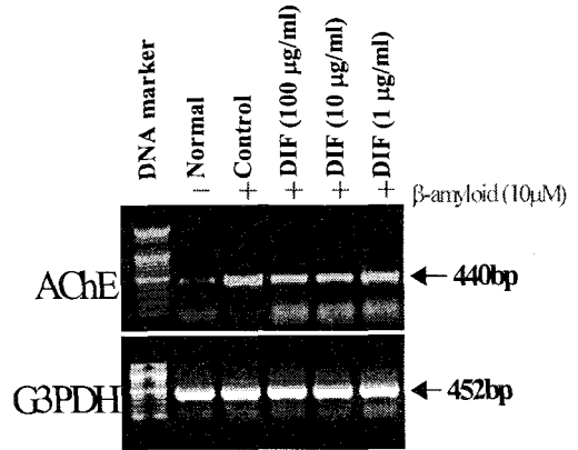
Fig. 3. Inhibitory effects of DIF extract on AChE mRNA expression in PC-12 cell cultures after treatment with A \beta . Normal : Non-treatment group. Control : Group pretreated with 10 \mu M A \beta for 1hr. DIF I : Group pretreated with 10 \mu M A \beta for 1 hour and 100 \mu g/ml of DIF extract for 6hrs. DIF II : Group pretreated with 10 \mu M A \beta for 1 hour and 10 \mu g/ml of DIF extract for 6hrs. DIF III : Group pretreated with 10 \mu M A \beta for 1 hour and 1 \mu g/ml of DIF extract for 6hrs. PC-12 cell line was pretreated with various concentration DIF extract(100, 10, 1 \mu g/ml) in the presence A \beta (10 \mu M) for 6hrs. Amplified PCR products were electrophoresed on 1.2% agarose gel, and the analysis(Ht) was used to 1D-density program. The other methods for assay were performed as described in Materials and Methods . The gene expressions were observed AChE mRNA expression, and internal control(G3PDH) in PC-12 cell line.
