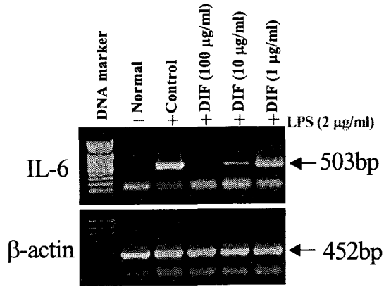
Fig. 6. Inhibitory effects of DIF extract on IL-6 mRNA expression in THP-1 cell line cultures after treatment with LPS. Normal : Non-treatment group. Control : Group pretreated with 2 \mu g/ml LPS for 1hr. DIF I : Group pretreated with 2 \mu g/ml LPS for 1hr and 100 \mu g/ml of DIF extract for 6hrs. DIF II : Group pretreated with 2 \mu g/ml LPS for 1hr and 10 \mu g/ml of DIF extract for 6hrs. DIF III : Group pretreated with 2 \mu g/ml LPS for 1hr and 1 \mu g/ml of DIF extract for 6hrs. THP-1 cell line was pretreated with various concentration DIF extract(100, 10, 1 \mu g/ml) in the presence LPS(2 \mu g/ml) for 6hrs. Amplified PCR products were electrophoresed on 1.2% agarose gel, and the analysis(Ht) was used to 1D-density program. The other methods for assay were performed as described in Materials and Methods . The gene expressions were observed IL-6 mRNA expression, and internal control( \beta -actin) in THP-1 cell line.
