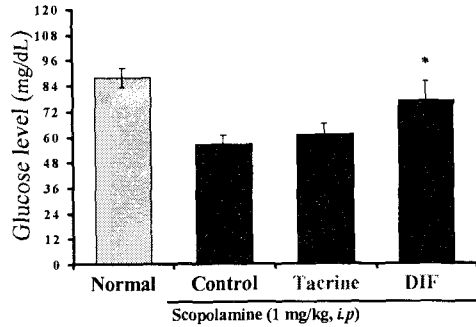
Fig. 9. Effects of DIF extract on the glucose in the serum level of memory deficit rats induced by scopolamine. Normal : Non-treatment group. Control : Group treated with scopolamine(1mg/kg i.p). Tacrine : Group treated with scopolamine(1mg/kg i.p) and tacrine(10mg/kg p.o). DIF : Group treated with scopolamine(1mg/kg i.p) and DIF extract(150mg/kg p.o). * : Statistically significant value compared with control data by T test(* : p<0.05, ** : p<0.01, *** : p<0.001). SD rats were orally administered with DIF or tacrine and the injection of scopolamine(1mg/kg i.p) continued once a day for 7 days. Hematologic change was analyzed as described in Materials and Methods .
