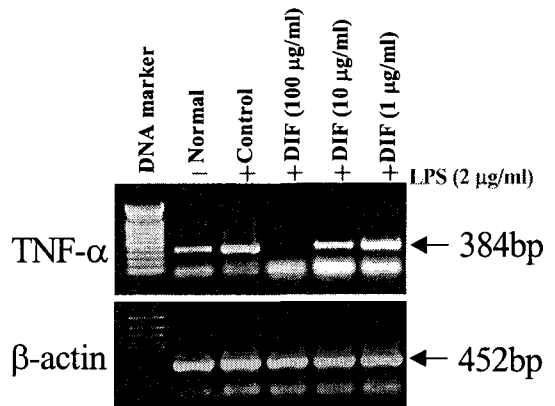
Fig. 7. Inhibitory effects of DIF extract on TNF- \alpha mRNA expression in THP-1 cell line cultures after treatment with LPS. Normal : Non-treatment group. Control : Group pretreated with 2 \mu g/ml LPS for 1hr. DIF I : Group pretreated with 2 \mu g/ml LPS for 1hr and 100 \mu g/ml of DIF extract for 6hrs. DIF II : Group pretreated with 2 \mu g/ml LPS for 1hr and 10 \mu g/ml of DIF extract for 6hrs. DIF III : Group pretreated with 2 \mu g/ml LPS for 1hr and 1 \mu g/ml of DIF extract for 6hrs. THP-1 cell line was pretreated with various concentration DIF extract(100, 10, 1 \mu g/ml) in the presence LPS(2 \mu g/ml) for 6hrs. Amplified PCR products were electrophoresed on 1.2% agarose gel, and the analysis(Ht) was used to 1D-density program. The other methods for assay were performed as described in Materials and Methods . The gene expressions were observed IL-6 mRNA expression, and internal control( \beta -actin) in THP-1 cell line.
