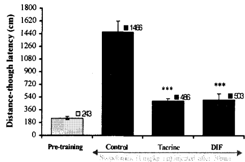
Fig. 13. Effects of DIF on the memory deficit mice induced by scopolamine in the distance movement-through type Morris water maze test.
