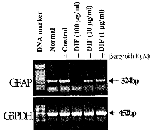
Fig. 4. Inhibitory effects of DIF extract on GFAP mRNA expression in PC-12 cell cultures after treatment with A \beta . Normal : Non-treatment group. Control : Group pretreated with 10 \mu M A \beta for 1hr. DIF I : Group pretreated with 10 \mu M A \beta for 1 hour and 100 \mu g/ml of DIF extract for 6hrs. DIF II : Group pretreated with 10 \mu M A \beta for 1 hour and 10 \mu g/ml of DIF extract for 6hrs. DIF III : Group pretreated with 10 \mu M A \beta for 1 hour and 1 \mu g/ml of DIF extract for 6hrs. PC-12 cell line was pretreated with various concentration DIF extract(100, 10, 1 \mu g/ml) in the presence A \beta (10 \mu M) for 6hrs. Amplified PCR products were electrophoresed on 1.2% agarose gel, and the analysis(Ht) was used to 1D-density program. The other methods for assay were performed as described in Materials and Methods . The gene expressions were observed GFAP mRNA expression, and internal control(G3PDH) in PC-12 cell line.
