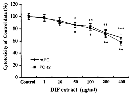
Fig. 1. Cytotoxicity of DIF extract on mLFC and PC-12 Cell line. Control : Non-treatment group. DIF : Group pretreated with various concentration(1µg/ml, 10µg/ml, 50µg/ml, 100µg/ml, 200µg/ml, 400µg/ml) of DIF extract for 48hrs. * : Statistically significant value compared with control data by T test(* : p<0.05, ** : p<0.01, *** : p<0.001).
