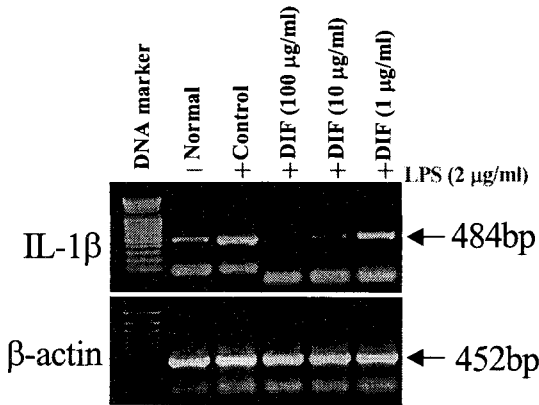
Fig. 5. Inhibitory effects of DIF extract on IL-1 \beta mRNA expression in THP-1 cell line cultures after treatment with LPS. Normal : Non-treatment group. Control : Group pretreated with 2 \mu g/ml LPS for 1hr. DIF I : Group pretreated with 2 \mu g/ml LPS for 1hr and 100 \mu g/ml of DIF extract for 6hrs. DIF II : Group pretreated with 2 \mu g/ml LPS for 1hr and 10 \mu g/ml of DIF extract for 6hrs. DIF III : Group pretreated with 2 \mu g/ml LPS for 1hr and 1 \mu g/ml of DIF extract for 6hrs. THP-1 cell line was pretreated with various concentration DIF extract(100, 10, 1 \mu g/ml) in the presence LPS(2 \mu g/ml) for 6hrs. Amplified PCR products were electrophoresed on 1.2% agarose gel, and the analysis(Ht) was used to 1D-density program. The other methods for assay were performed as described in Materials and Methods . The gene expressions were observed IL-1 \beta mRNA expression, and internal control( \beta -actin) in THP-1 cell line.
