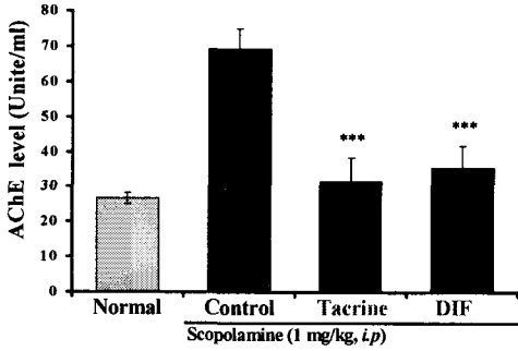
Fig. 11. Effects of DIF extract on the AChE in the serum level of memory deficit rats induced by scopolamine.
