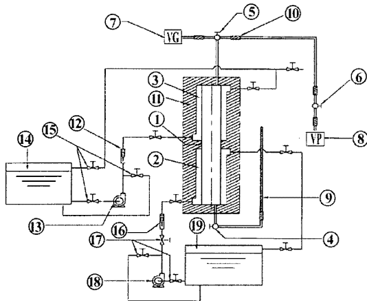
1. Test Tube 2. Heating Water Chamber 3. Cooling Water Chamber 4. Vacuum Valve 5. Vacuum Valve 6. Vacuum Rubber Hose 7. Vacuum Gauge 8. Vacuum Pump 9. Measuring Device for Liquid Level 10. Vacuum Rubber Hose 11. Insulation 12. Coolant Flow Meter 13. Coolant Pump 14. Coolant Constant Temperature Bath 15. Coolant Control Valve 16. Heating Water Flow Meter 17. Heating Water Control Valve 18. Heating Water Pump 19. Heating Water Constant Temperature Bath
