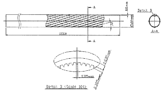
Fig. 2 Cross-sectional view of helical grooved thermosyphon
