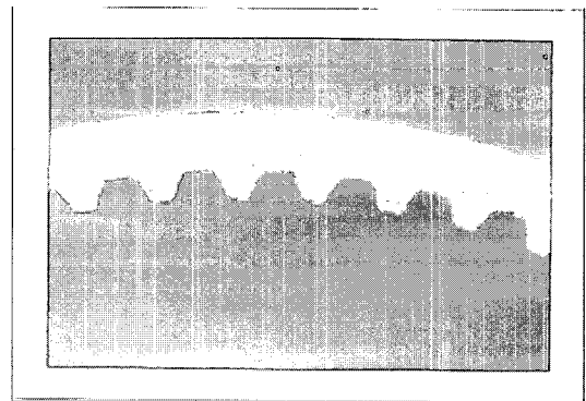
Fig. 3 Enlarged cross-sectional view of internal grooves (60 grooves)
