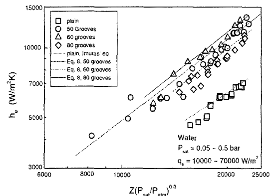
Fig. 9 Comparison of the experimental results with equations (4) and (8) for water
