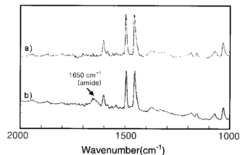
Figure 3. ATR-FTIR spectra of ungrafted (a) and PIPAAm grafted (b) cell culture surfaces.
