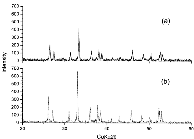
Fig. 7. X-ray diffraction patterns for nacre of cultured pearl used (a) the bead nucleus made from washboard shell and (b) bio bead nucleus developed in the study.
