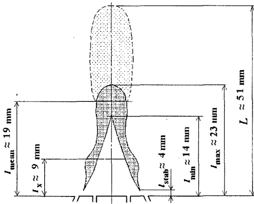
Fig. 9 Photograph and schematic of the flames formed for one operating condition of lower instability region ( q=U_o/U_r\sqrt{\rho_o/\rho_f}=0.41 and U_o=18.51 m/s)
