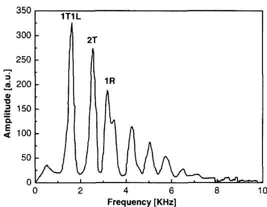
Fig. 6 Amplitude spectrum for stable combustion
