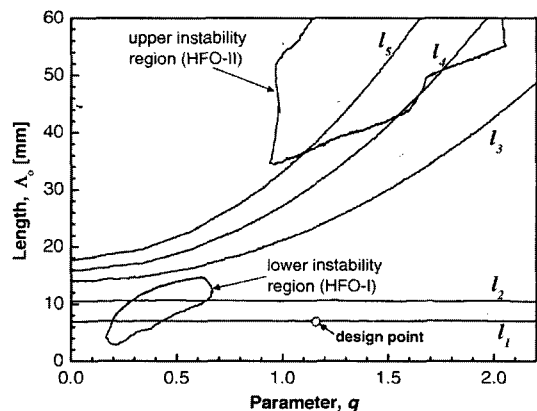
Fig. 13 Stability boundaries plotted on the coordinate of disturbance-wave length, \Lambda_o vs. q
