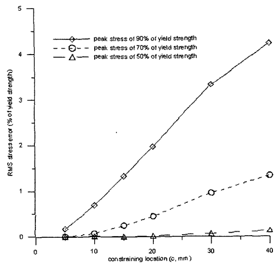
Fig. 7 RMS stress error averaged through the plane of the cut
