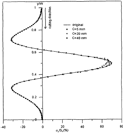
Fig. 5 Recomputed residual stress distributions by the contour method when the peak value of original stress is 70% of the yield strength
