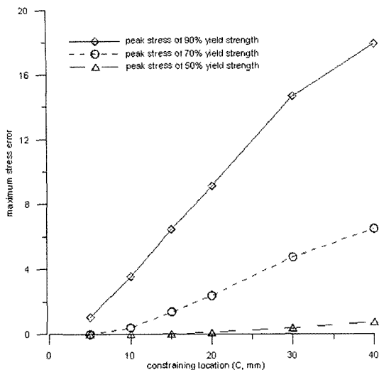
Fig. 8 Maximum stress error along the plane of the cut
