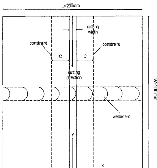
Fig. 1 Schematic of the contour method on an Alloy C-22 welded plate
