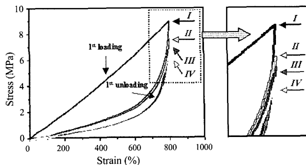
Figure 8. Stress-strain curves of electrospun TPUE fiber mats for various cycles under fixed strain of 800%.
