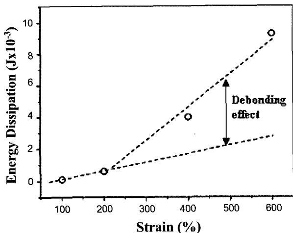
Figure 6. Energy dissipation of electrospun TPUE fiber mats under different strains.
