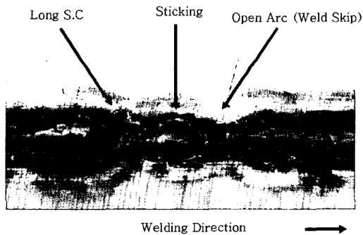
Fig. 7 Bead appearance formed by stubbing at the high speed CO 2 welding
