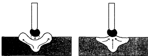
(a) Arc (b) Short circuit
