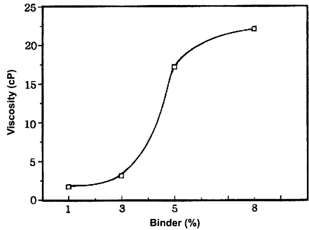
Fig. 3. Variation of viscosities with binder contents.
