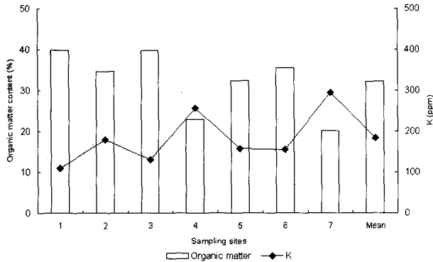
Fig. 1. Mean contents of soil organic matter and K collected from seven different Lepista nuda habitats. 1. Incheon Mt. Mani, 2. Incheon Bupeong, 3. Gyeonggi Kimpo, 4. Gyeonggi Yongin, 5. Jeonbuk Mt. Deogyu, 6. Gyeongbuk Gyeongsan, 7. Gyeongbuk Hayang.
