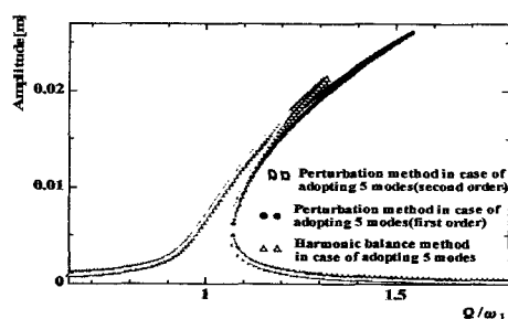
Fig. 4 Comparison of frequency responses
