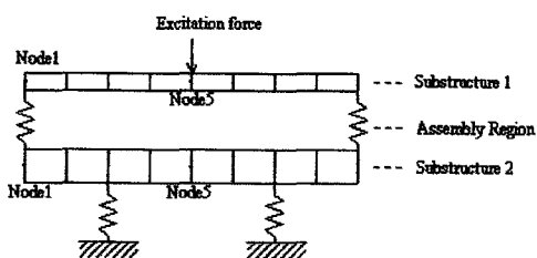
Fig. 2 Model for analysis
