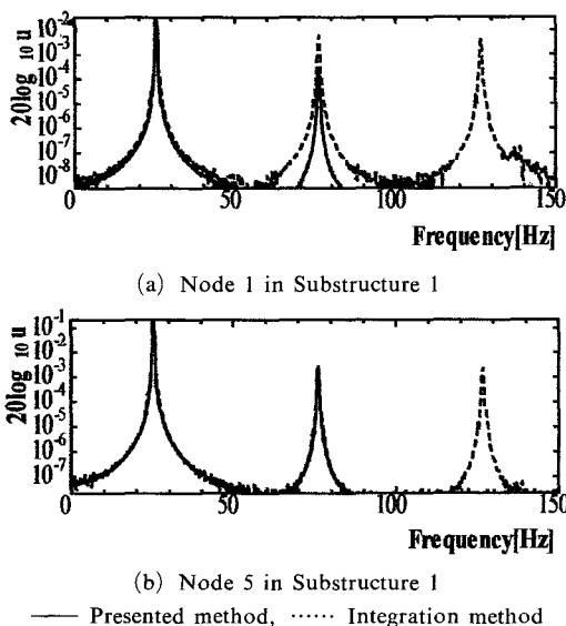
Fig. 8 Comparison of Frequency Spectra
