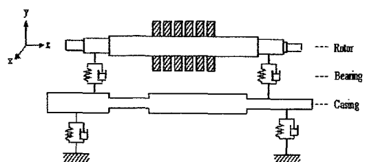
Fig. 1 Rotor-bearing-casing system
