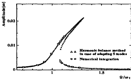
Fig. 5 Comparison of frequency responses
