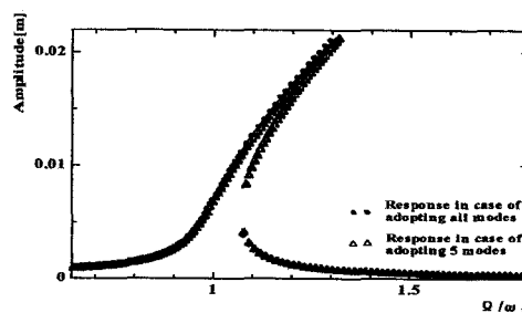
Fig. 3 Effect of adopting modes in frequency response
