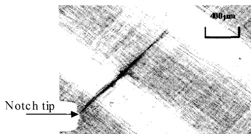
Fig. 14 Polarized optical microscopy observation of fracture processes in a satin-weave -[+45 0 / 45 ] 16 composite specimen around 95% of P_{max} under transmitted light.
