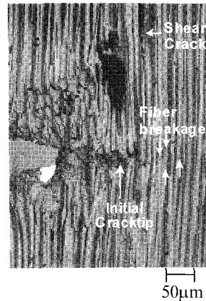
Fig. 9 Reflected optical micrograph of notched UD- [0^0_8]_s specimen in load stage II of Fig. 8.
