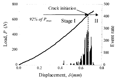
Fig. 11 Typical diagrams of load P and AE event rate versus displacement \delta for a satin weave [0°/90°] 16 composite specimen. AE event rate data was obtained from high amplitude signals beyond 70 dB.
