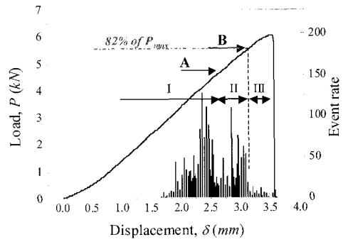
Fig. 8 Typical diagrams of load P and AE event rate versus displacement \delta for notched [0^0_8]_s composite specimen: Accompanying AE event rate data was obtained with high amplitudes beyond 70 dB.
