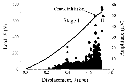
Fig. 12 Behavior of the AE amplitude distribution versus \delta for the specimen of Fig. 11. The amplitude data was obtained from all AE signals beyond the threshold level (40 dB).
