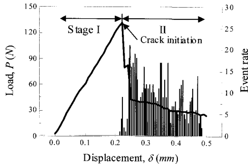
Fig. 5 Typical diagrams of load P and AE event rate versus displacement \delta for the same specimen as used in Fig. 3: Accompanying AE event rate data was obtained from signals with high amplitudes beyond 70 dB.
