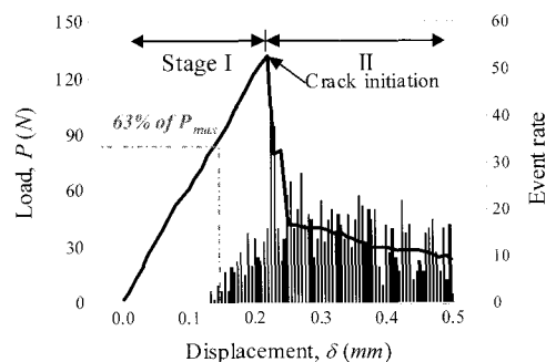
Fig. 3 Typical diagrams of load P and AE event rate versus displacement \delta for unidirectional [90°] 8 composite specimen: Accompanying AE event rate data was obtained from signals with low and intermediate amplitudes from 40 to 70 dB.
