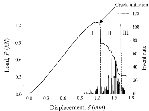
Fig. 10 Typical diagrams of load P and AE event rate versus displacement \delta for [+45^0_4/-45^0_4]_s composite specimen. Accompanying AE event rate data was obtained with high amplitudes beyond 70dB.
