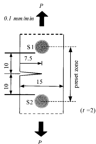
Fig. 1 Notched specimen of composite laminates and AE sensor locations S1 and S2.
