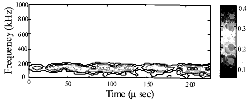
Fig. 4 A weak AE signal processed by the short time Fourier Transform with low frequency bands.
