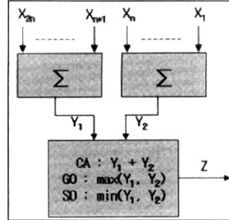
Fig. 4. Block Diagram of OS-CFAR
