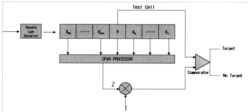
Fig. 2. Block Diagram of CFAR Process
