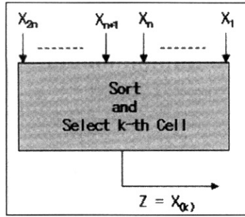
Fig. 3. Block Diagram of Mean Level CFAR
