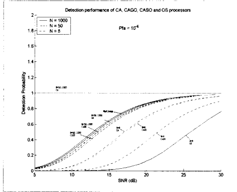
Fig. 6. Detection Probability of CA, GO, SO, and OS-CFAR
