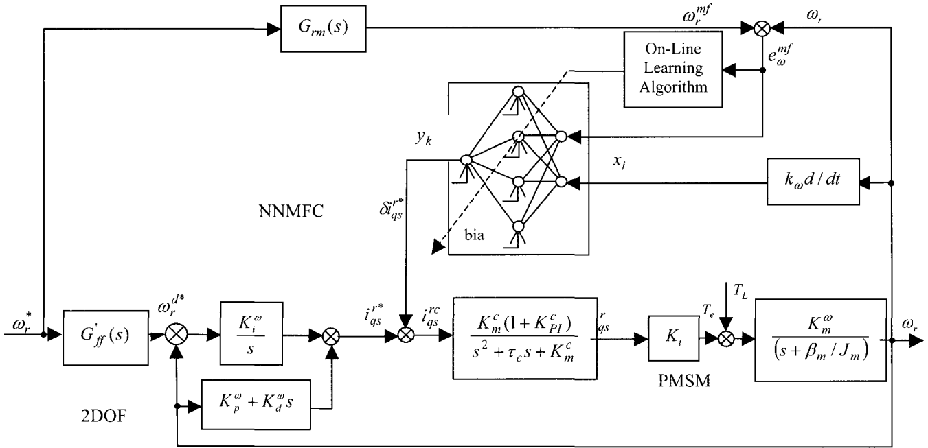
Fig. 2 Configuration of the proposed NNMFC speed controller for a field oriented PMSM drive system
