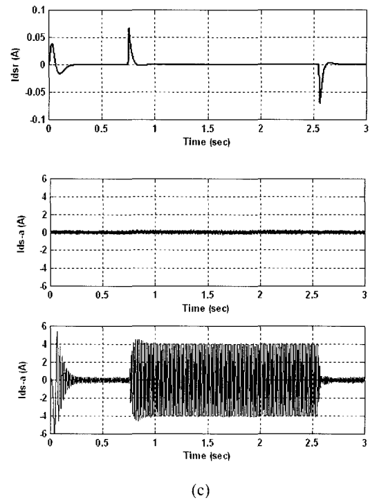
Fig. 6 Step speed response of a PMSM drive system using a 2DOF I-PD speed controller (a) Speed and torque responses. (b) Reference and actual q -axis stator current responses (c) Reference and actual d -axis stator current responses
