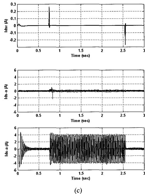
Fig. 7 Step speed response of a PMSM drive system using a 2DOF I-PD NNMF speed controller (a) Speed and torque responses. (b) Reference and actual q-axis stator current responses (c) Reference and actual d-axis stator current responses
