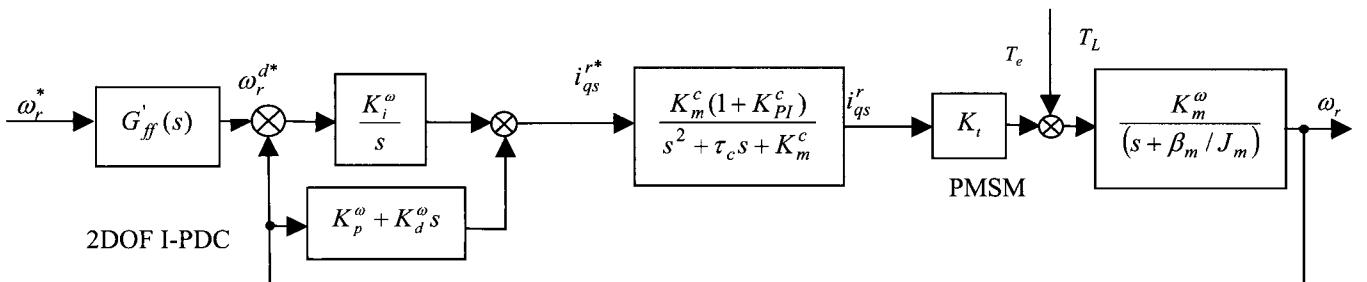
Fig. 4 Configuration of the speed control for PMSM using 2DOF I-PD speed controller
