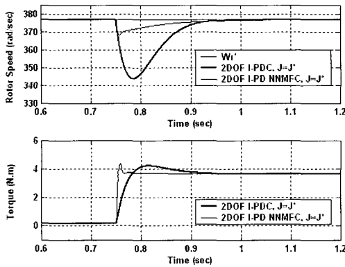
Fig. 8 The load regulation performance for both speed controllers with nominal parameters
